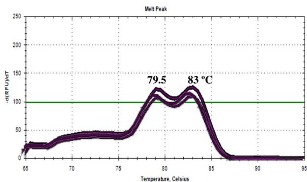
Fig. 7 Representative melting curve analysis profile obtained by multiplex with 66 pg/μL gDNA of R. arrhizus (79.5 °C) and 66 pg/μL gDNA of A. niger (83 °C) (n = 3)
