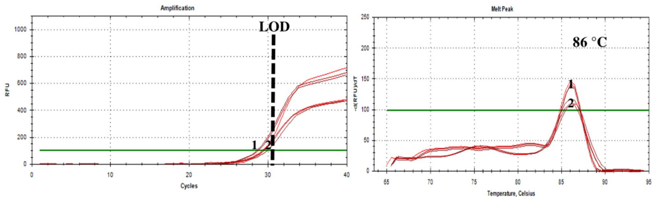
Fig. 10 Representative amplification curve profiles and melting curve analysis profiles obtained by multiplex with: (1) 0.06 ng/μL; (2) 0.03 ng/μL, gDNA of A. terreus (86 °C) ( n = 3 )
