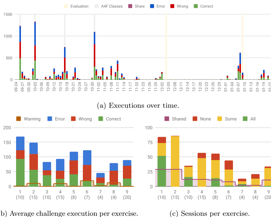
Fig. 3: Alloy4Fun usage statistics by 17 students over a semester for 9 exercises.
