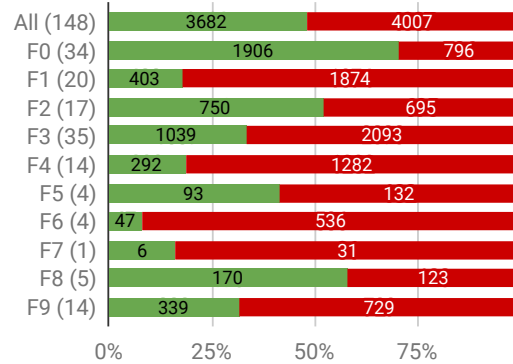
Fig. 4: Executions per class of challenge.
