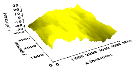
Fig.1. Microtopography of an asphalt mixture.
