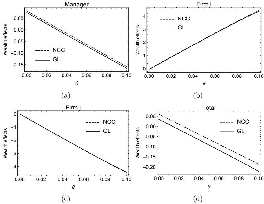
Figure 10: A sensitivity analysis for the effect of the value loss/gain to firm i/j ( \theta ) caused by the departure of the manager from firm i to firm j on the wealth.
