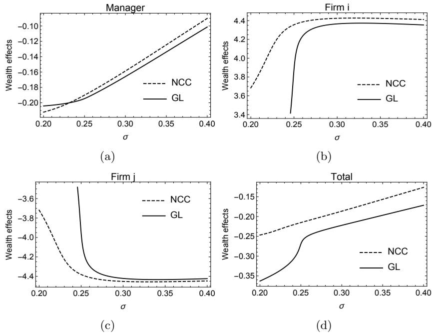
Figure 9: A sensitivity analysis of the effect of uncertainty ( \sigma ) on the wealth.
