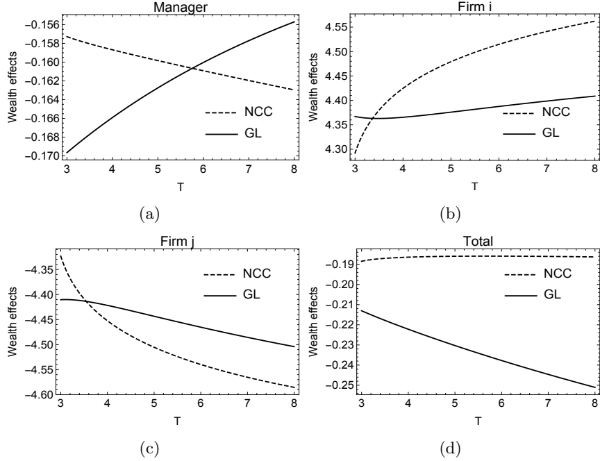
Figure 8: A sensitivity analysis of the effect of the embargo period ( T ) on the wealth.
