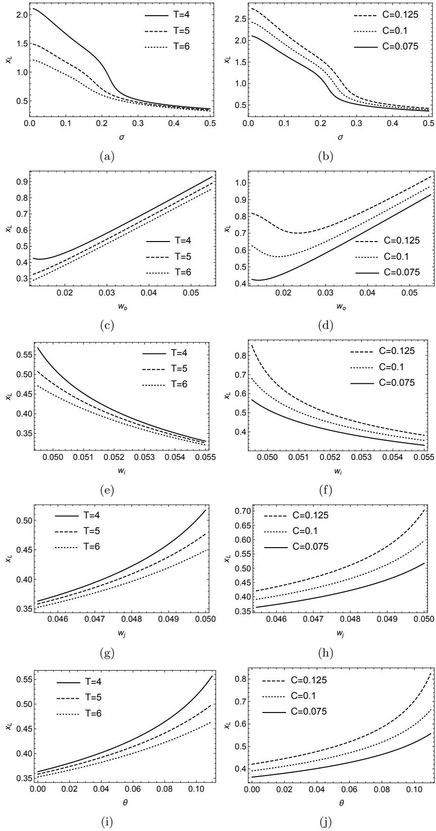
Figure 3: A sensitivity analysis for the effect of our model parameters on the optimal threshold to leave firm i ( x_L ), for a non-compete covenant (NCC).
