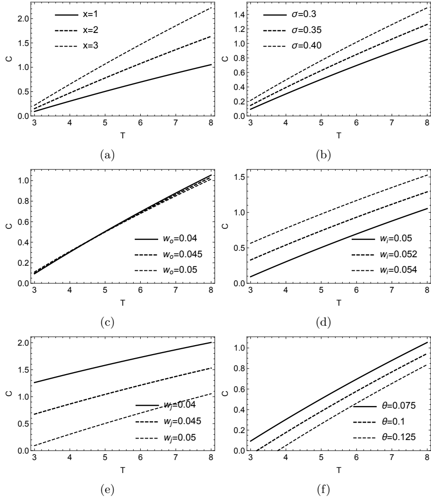
Figure 4: A sensitivity analysis for the effect of our model parameters on the optimal severance payment ( C ) versus embargo period ( T ) pair values, for a non-compete covenant (NCC).
