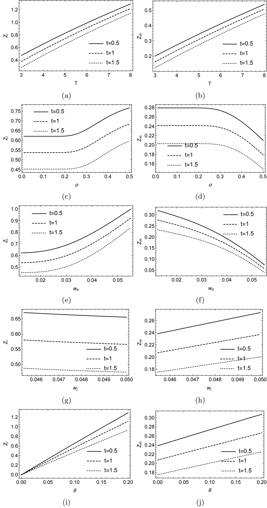
Figure 5: A sensitivity analysis for the effect of our model parameters on the value loss of the firm i ( Z_i ) and the value gain of the manager ( Z_m ), when the manager is tied to a non-competitive covenant (NCC) and there is a violation of the embargo period of the contract.
