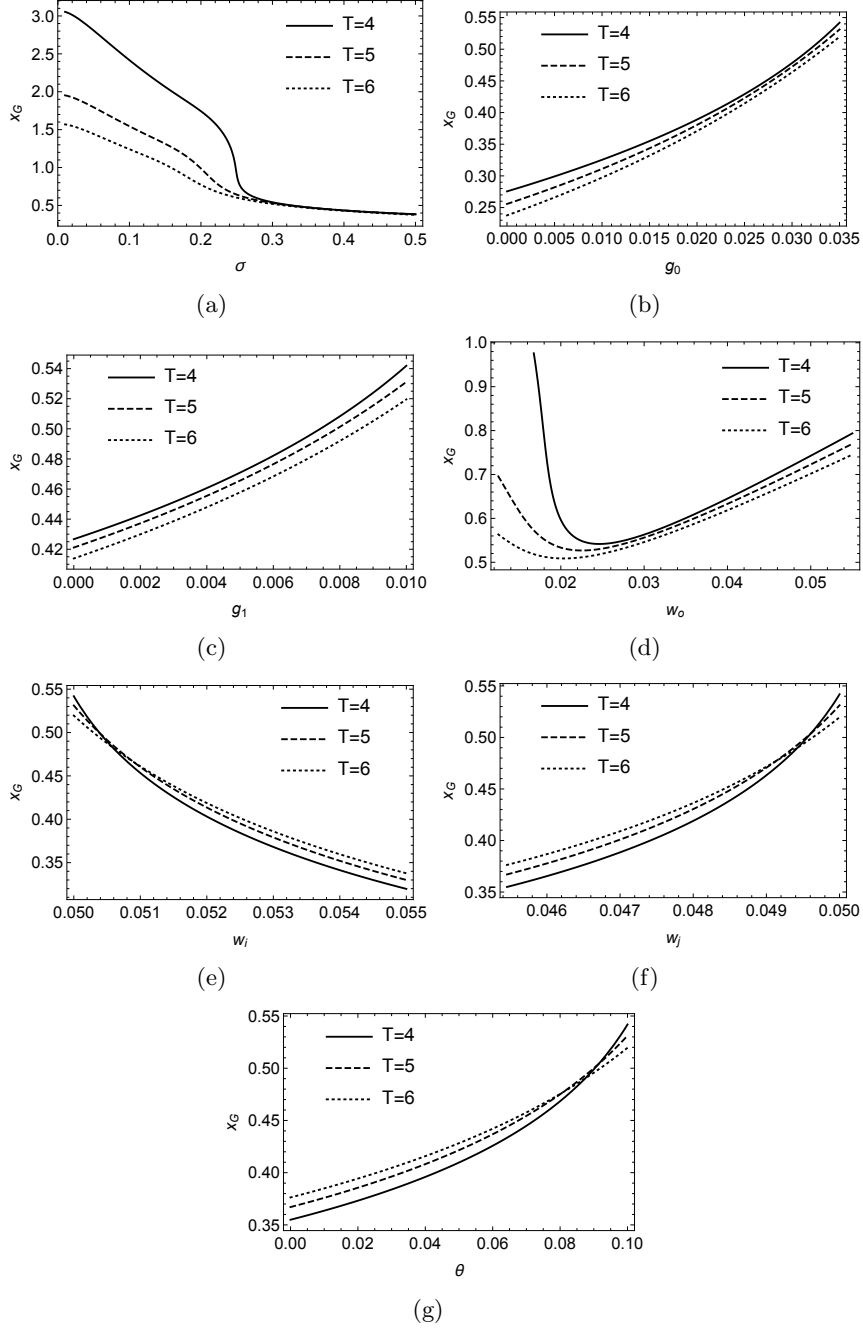
Figure 6: A sensitivity analysis for the effect of our model parameters on the optimal threshold to leave firm i ( x_G ) if the manager is tied to a garden leave (GL).
