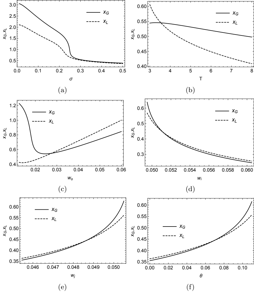
Figure 7: A comparative sensitivity analysis between a non-compete covenant (NCC) and a garden leave (GL), regarding the effect of our model parameters on the optimal thresholds to leave firm i .
