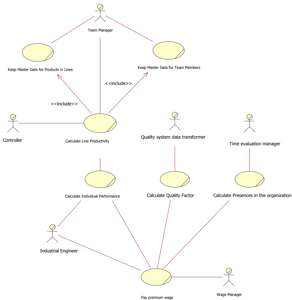
Fig. 4: Business use case model – To-Be situation.
