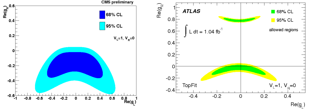
Figure 1: CMS(left) and ATLAS(right) allowed regions, at 68% and 95% CL, on the anomalous coupling plane (g_L, g_R) , for V_R=0 and V_L=1 .
