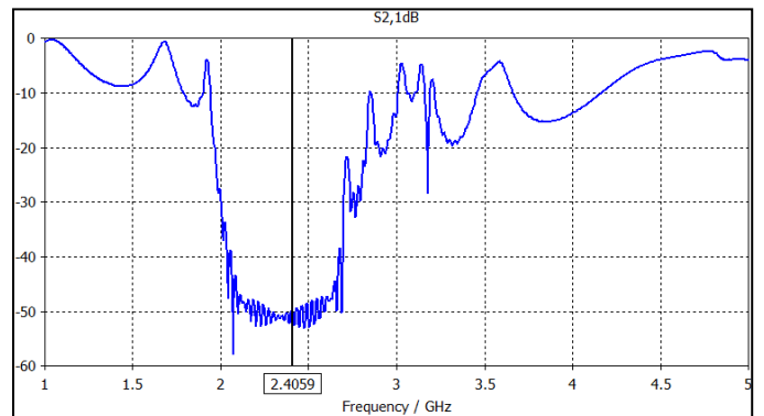
Fig. 4. S21 results when using superstrat.
