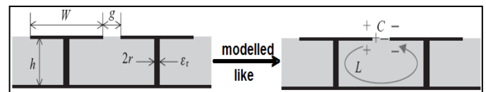
Fig. 1. The electrical equivalent circuit of EBG cells.
