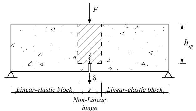
Fig. 12 - Specimen idealisation for model use.
