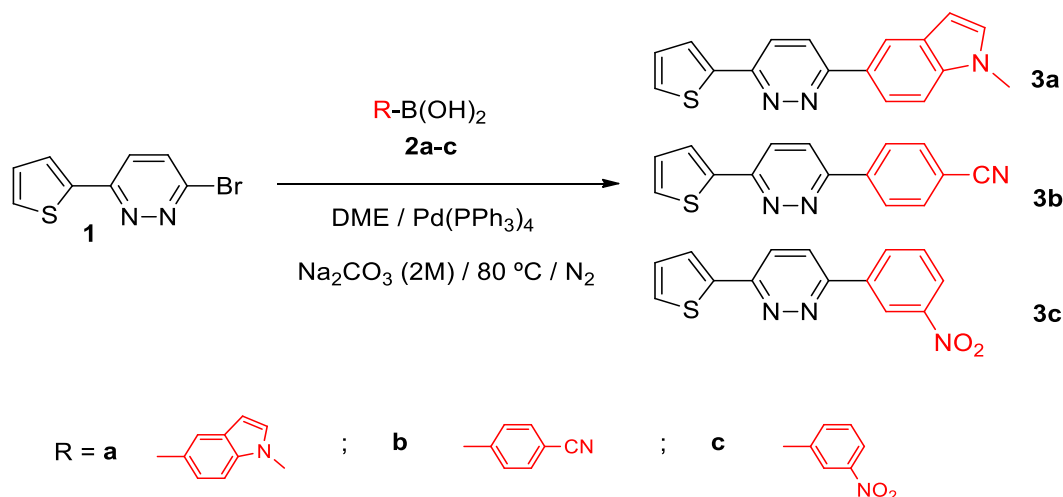
Scheme 1. Synthesis of thienyl-pyridazine derivatives 3 .
