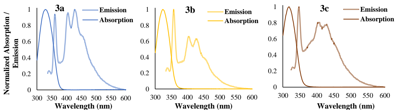
Figure 1. UV-Visible absorption and emission spectra of the novel thienyl-pyridazines 3 in ethanol solution.
