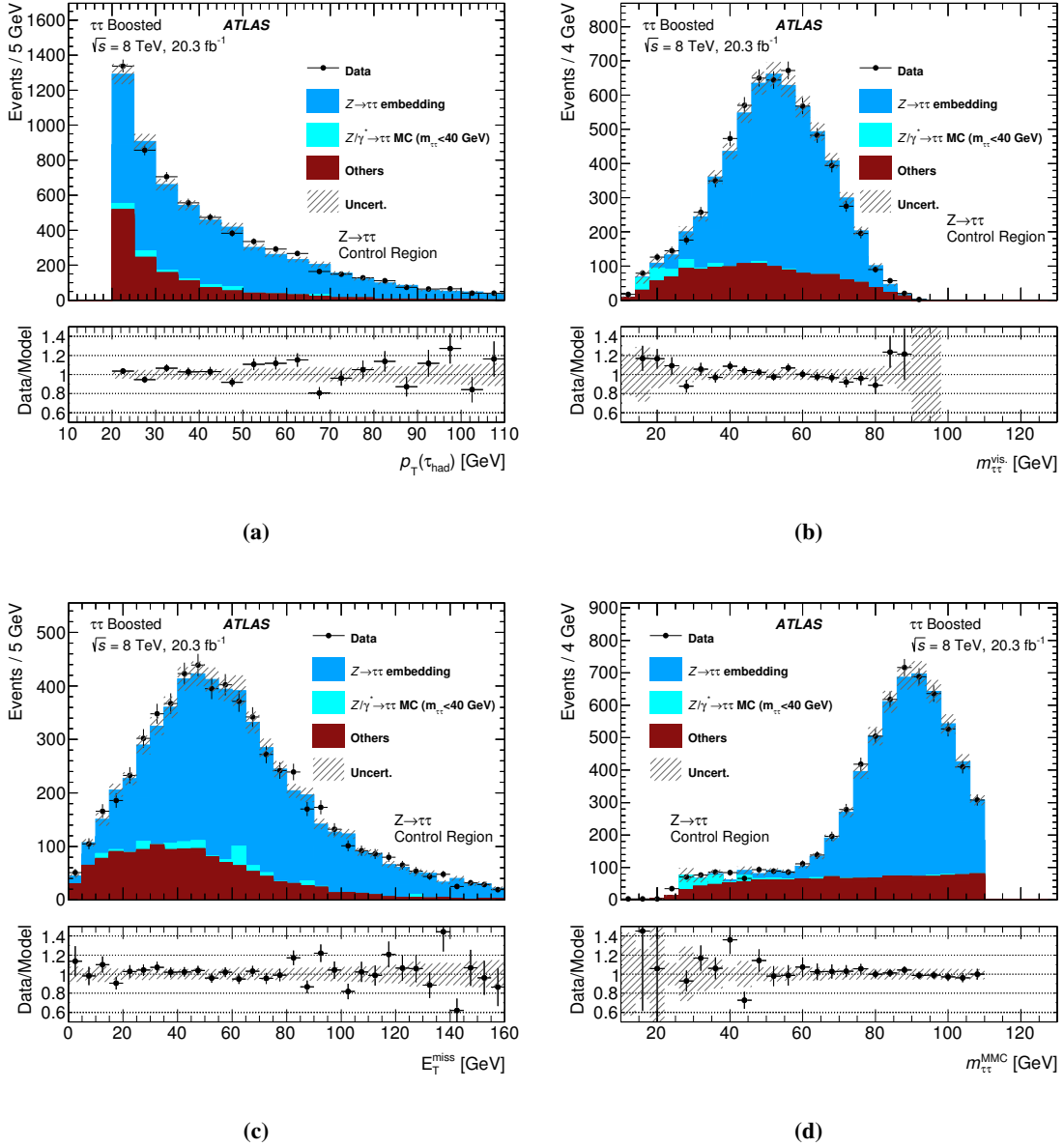
Figure 12. Comparison of data with the combined background model for example observables in the boosted Z -enriched control region: (a) \tau_{\text{had}} transverse momentum, (b) invariant mass of the visible \tau\tau decay products (c) missing transverse momentum and (d) the \tau\tau invariant mass obtained with the MMC, each including ratios showing the relative differences of the data to the total background estimate. The background contributions from other processes and the systematic uncertainties are estimated as described in ref. [1].
