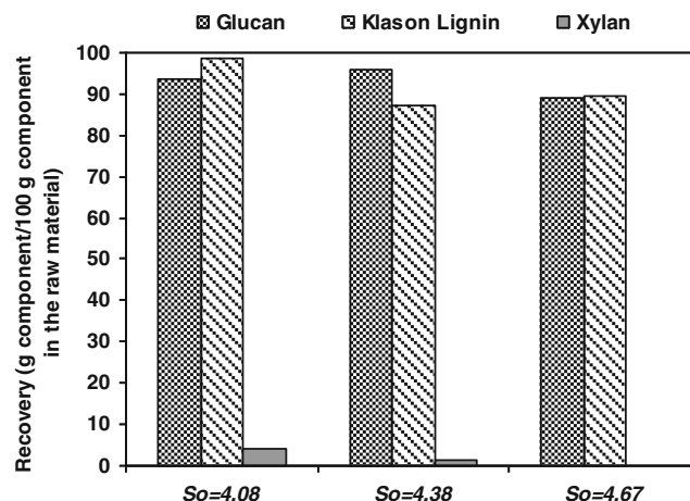
Fig. 2 Recovery of main components in the pretreated solid (on dry basis) after autohydrolysis process
