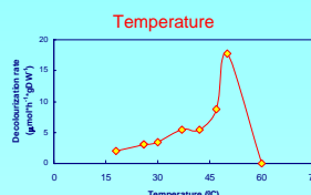
Figure 5: Effect of the temperature on the decolourisation rate.
