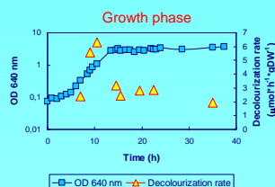
Figure 4: Effect of the growth phase on the decolourisation rate.
