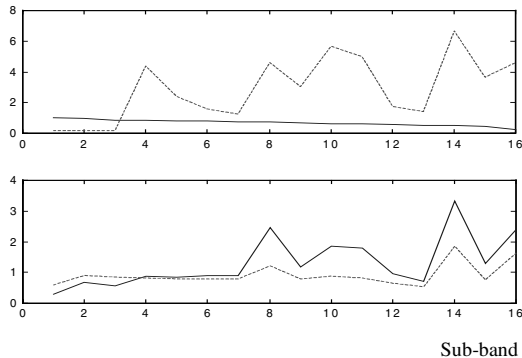
Figure 1. Upper: true (line) and initial channel estimate. Lower: first (line) and second channel estimates. The initial noise estimate was 10^5 times the true value for mean and variance.
