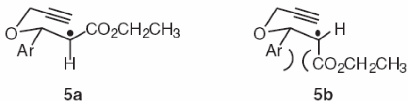
Fig. 2 Conformations of radical 4 .
