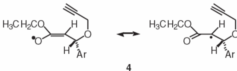
Fig. 1 Resonance forms of radical 4 .
