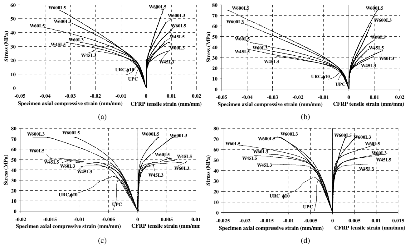
Fig. 8. Influence of confinement arrangement type on G3_RC group of test series: (a) C16S200 \phi 10; (b) C16S300 \phi 10; (c) C32S200 \phi 10; (d) C32S300 \phi 10.
