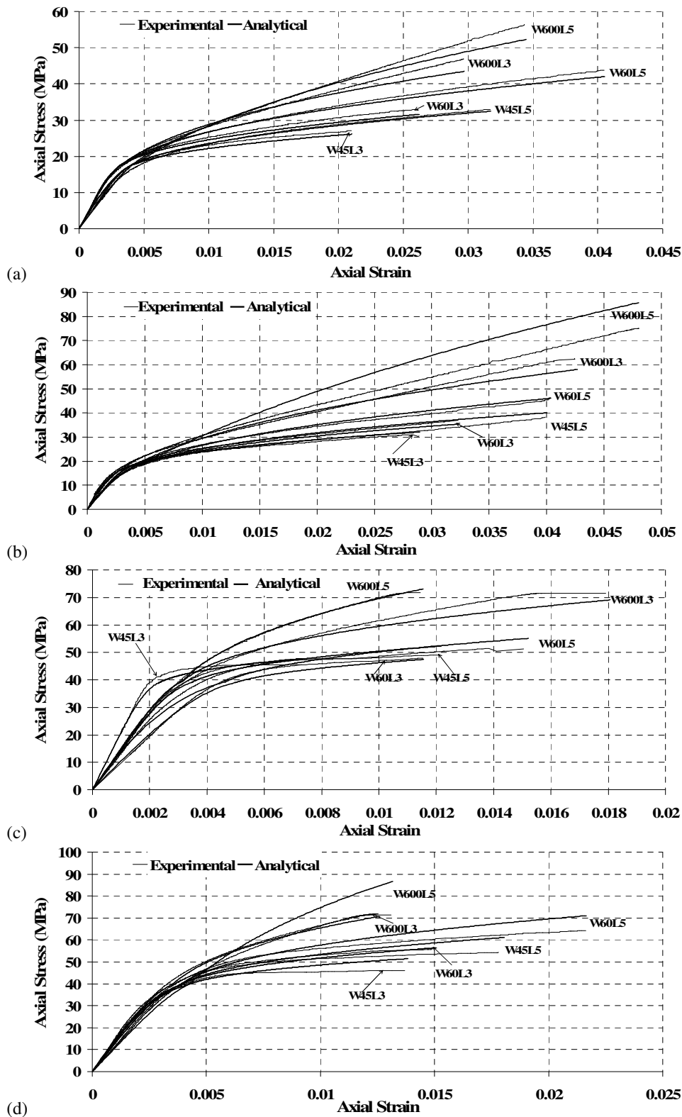
Fig. 12. Comparison between analytical model and experimental results for the: (a) C16S200φ10; (b) C16S300φ10; (c) C32S200φ10; (d) C32S300φ10.
