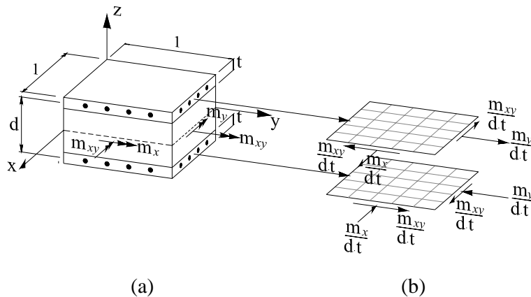
Figure 2.1 – Sandwich model of two layers: a) definition; b) membrane outer layers with resulting in-plane stresses
