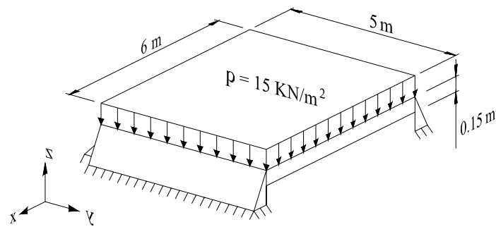
Figure 5.3 – Geometry and loads for simply supported slab
