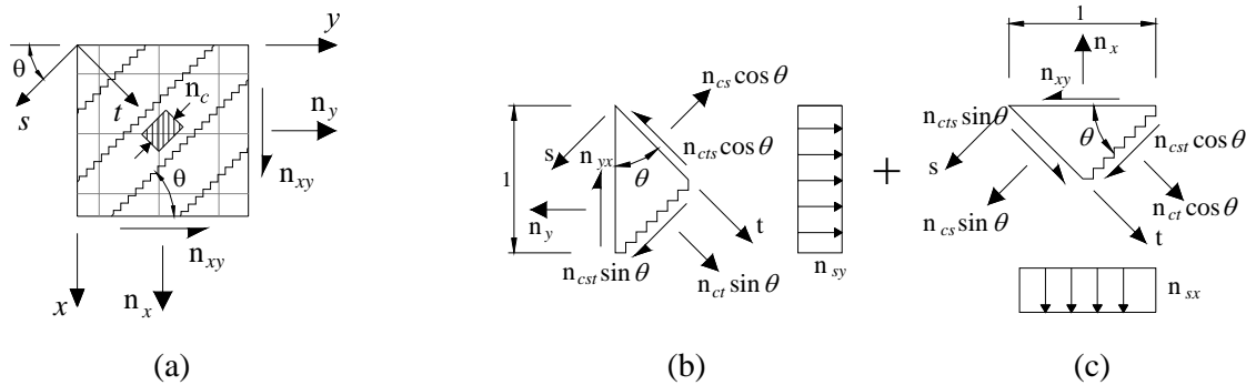
Figure 3.1 – Cracked membrane: a) notation; b) and c) forces at crack.
