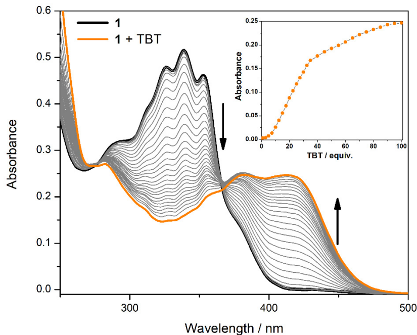
Figure 2. Spectrophotometric titration of thiosemicarbazone 1 with TBT.
