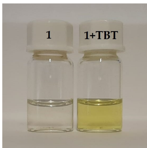
Figure 1. Preliminary TBT chemosensory test for the new thiosemicarbazone 1 : left—compound 1 ; right—compound 1 + 50 equivalents of TBT.
