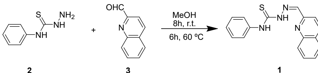
Scheme 1. Synthesis of thiosemicarbazone 1 .
