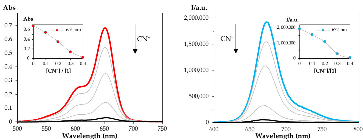
Figure 4. Spectrophotometric (left) and spectrofluorimetric (right) titration of probe 1 with \text{CN}^- in acetonitrile solution: [\mathbf{1}] = 5.0 \times 10^{-6} M. Inset: absorption at 651 nm and emission at 672 nm as a function of added anion equivalents.
