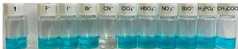
Figure 2. Colorimetric responses of probe 1 in acetonitrile solution ( 1.0 \times 10^{-5} M) before and after the addition of 20 equiv. of various anions.
