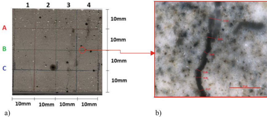
Fig. 3 a Scheme for measuring of the crack number and widths; b Typical photo with measurements of crack width
