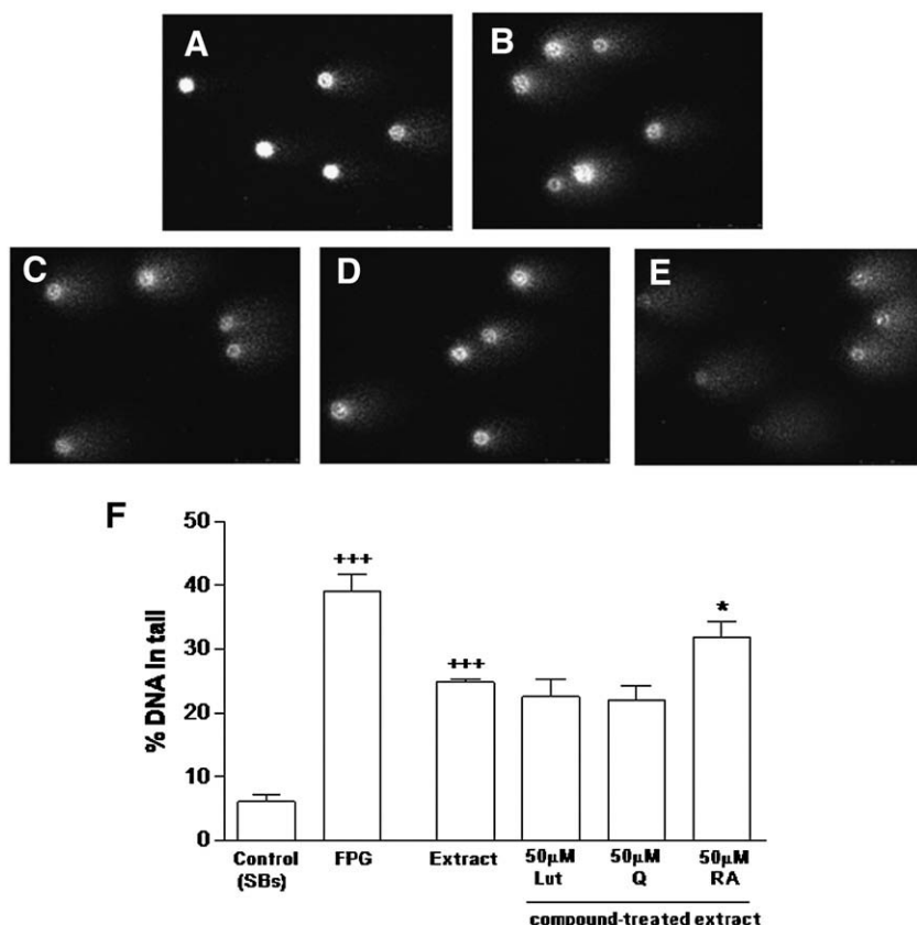
Fig. 11. Effect of the compounds on the in vitro BER assay. A–E) representative images of Comets (purines only) from control (buffer alone), extract from non-treated cells, extract from 50 \mu M luteolin-treated cells, extract from 50 \mu M quercetin-treated cells and extract from 50 \mu M rosmarinic acid-treated cells, respectively. F) Quantification of the percentage of DNA in the comet tails was done after treatment of damage-containing substrate cells with a cell-free extract obtained from PC12 cells incubated with the polyphenols for 24 h. The repair enzyme FPG was used as a positive control. Levels of oxidized purines were determined and quantified as previously described. For each condition is represented the mean \pm S.E.M for at least three independent experiments. *** P \leq 0.001 compared to control cells; * P \leq 0.05 , relatively to non treated extract. SBs – Strand Breaks.
