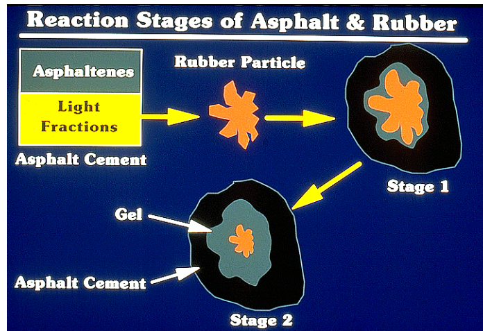
Figure 4 – Interaction between asphalt rubber and asphalt (Holleran and Reed, 2000)
