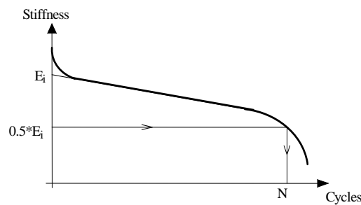
Figure 8 – Stiffness evolution during fatigue tests and definition of test failure
