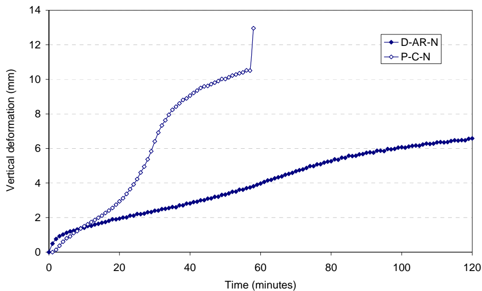
Figure 12 – Permanent deformation resistance
