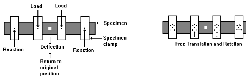
Figure 6 – Schematic representation of the four point test setup
