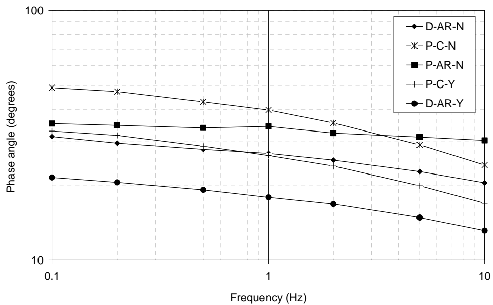
Figure 10 – Phase angle of the studied mixtures
