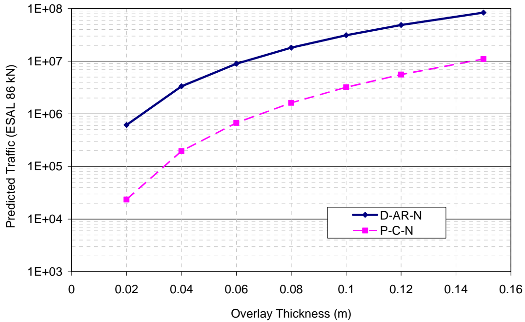
Figure 13 – Estimation of overlay life
