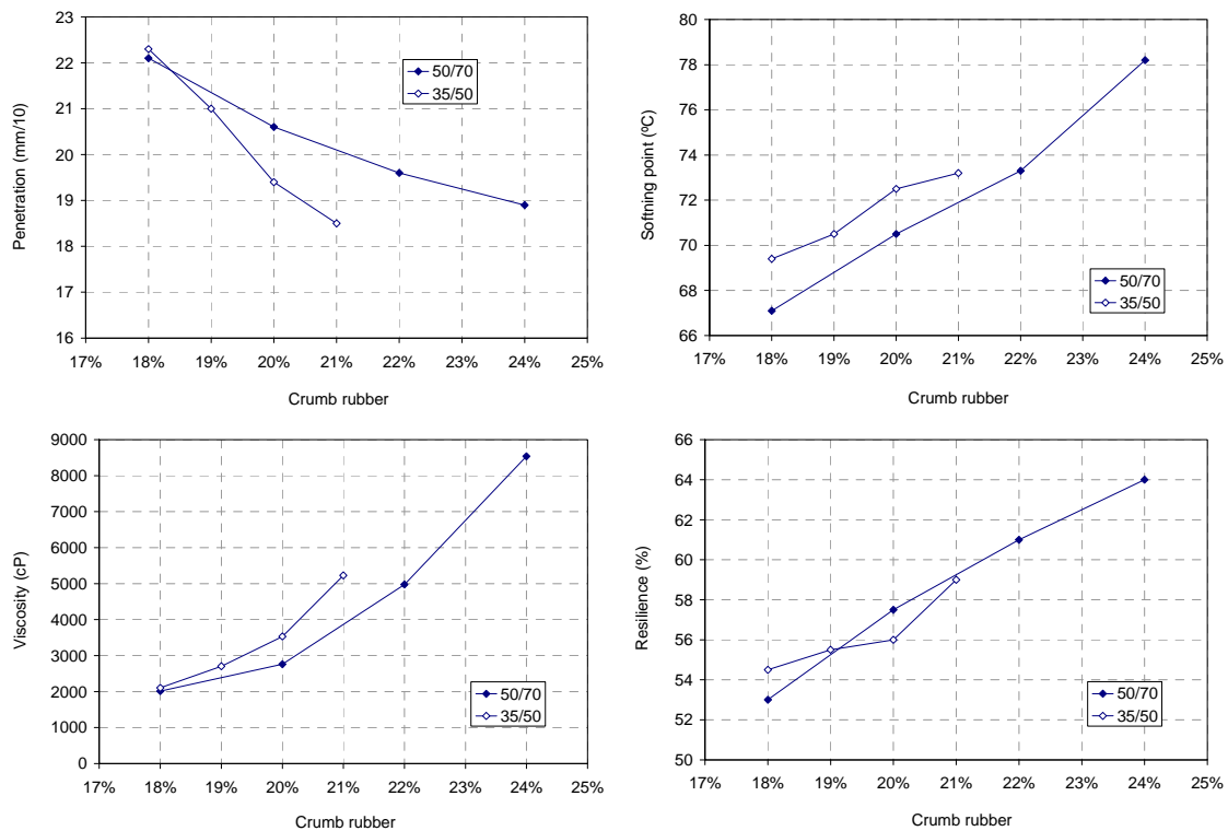
Figure 5 – Influence of crumb rubber content on the asphalt rubber characteristics
