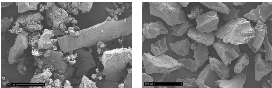
Figure 2 – Ambient crumb rubber (left) cryogenic crumb rubber (right)
