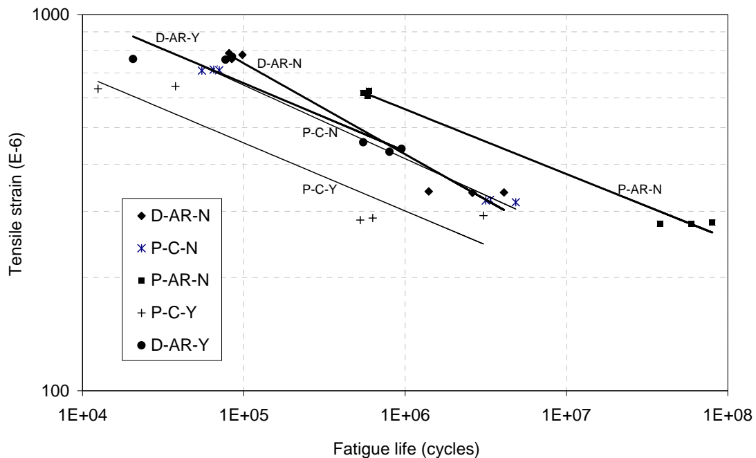
Figure 11 – Fatigue curves of the studied mixtures
