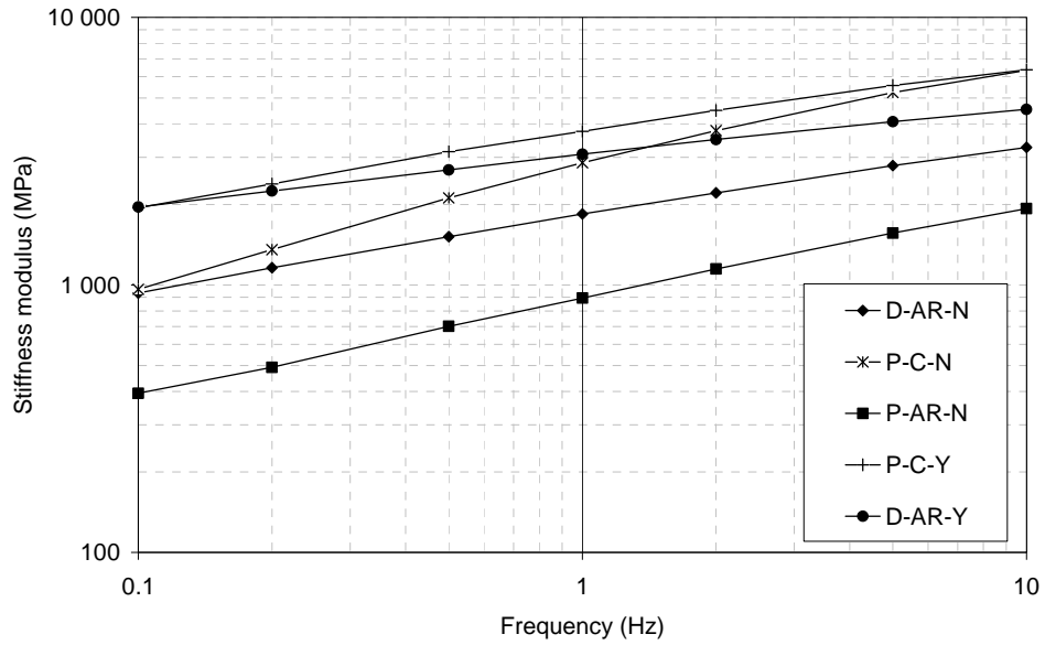
Figure 9 – Stiffness modulus of the studied mixtures
