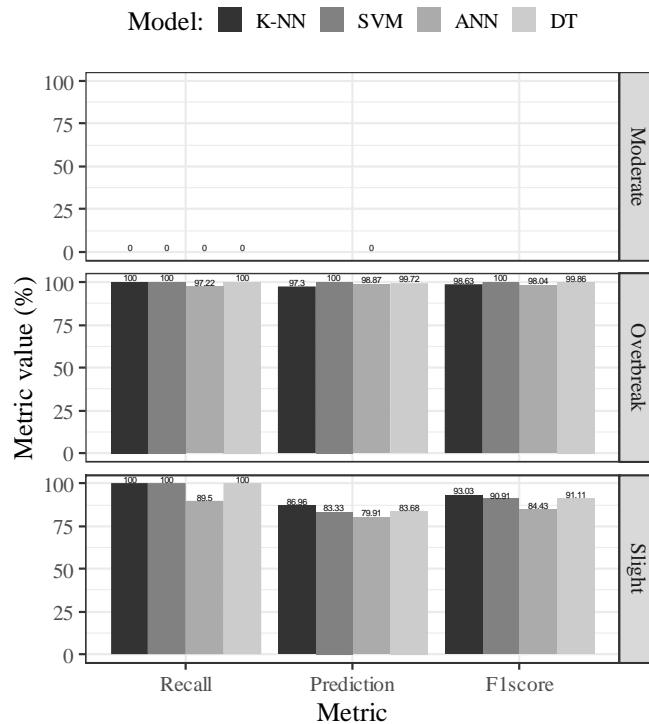
Figure 6: Comparison of DM models' performance for in situ rockburst prediction based on recall, precision, and F_{1-score} metrics.
