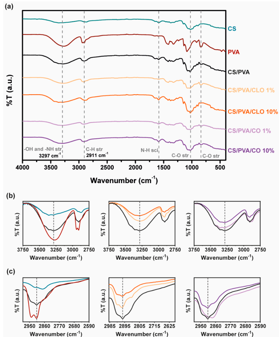
Figure 4. (a) FTIR-ATR spectra of the EO-unloaded and loaded CS/PVA-based blended films ( 4000\text{--}400\text{ cm}^{-1} ). Sections between (b) 3750\text{--}2750\text{ cm}^{-1} and (c) 2990\text{--}2590\text{ cm}^{-1} were amplified for a clearer detection of the most relevant peaks.
