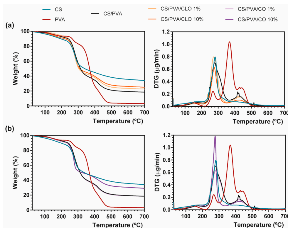
Figure 5. Representative TGA (left) and DTG (right) curves of (a) CLO- and (b) CO-loaded CS/PVA blended films, and respective controls from 25 to 700 °C, performed at a heating rate of 10 °C/min in a nitrogen atmosphere.
