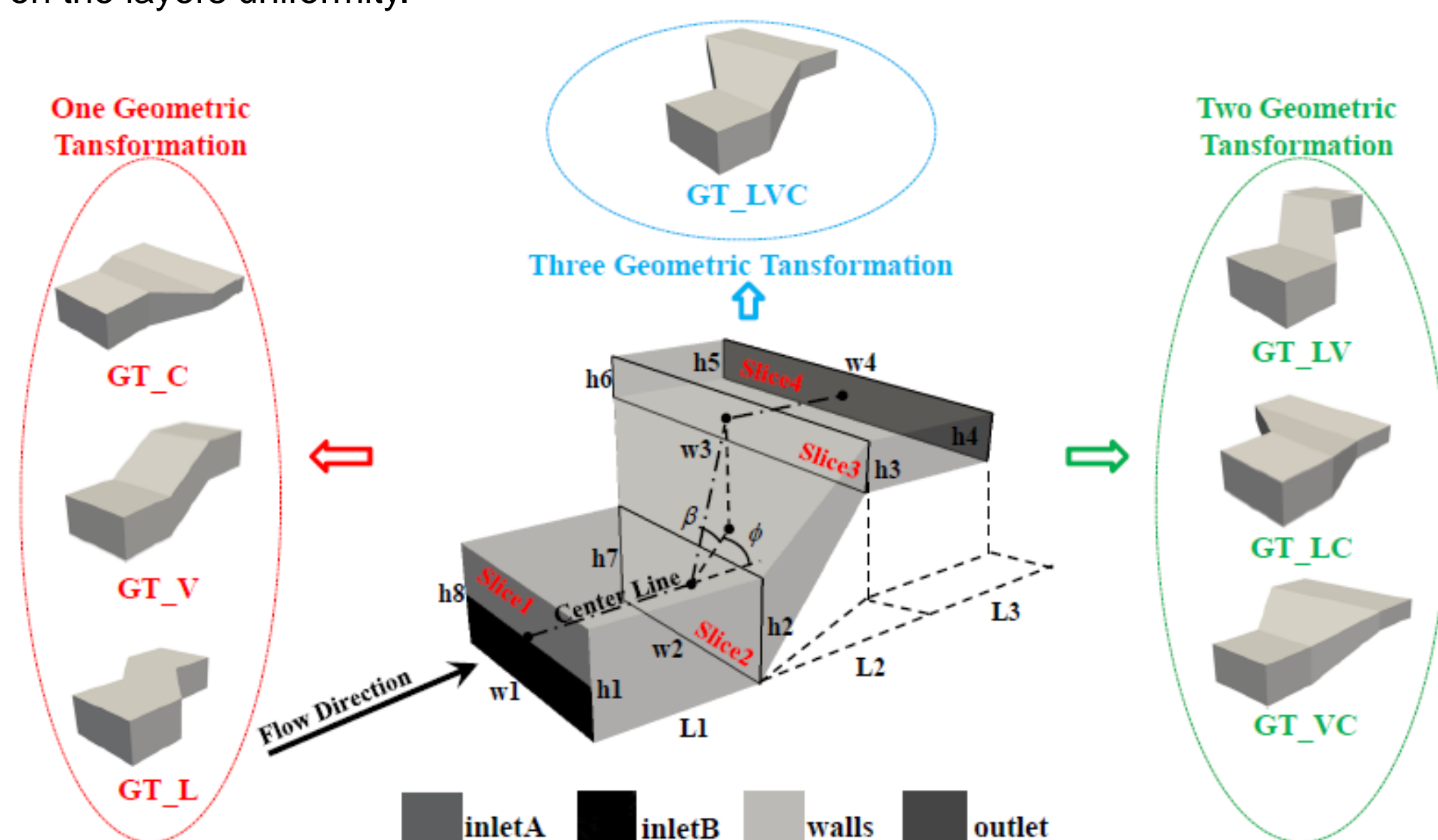
Figure 4. All GTs identified and base geometry to be used on the GT study.
