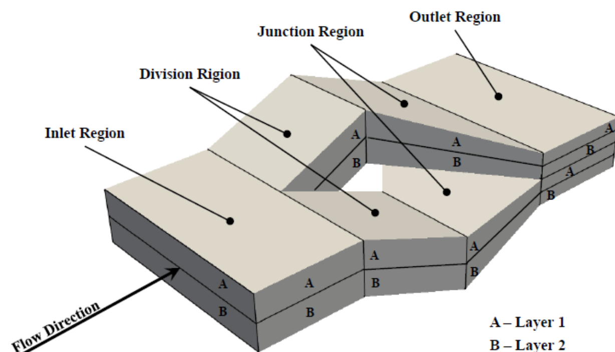
Figure 1. Interfacial surface generator module.
