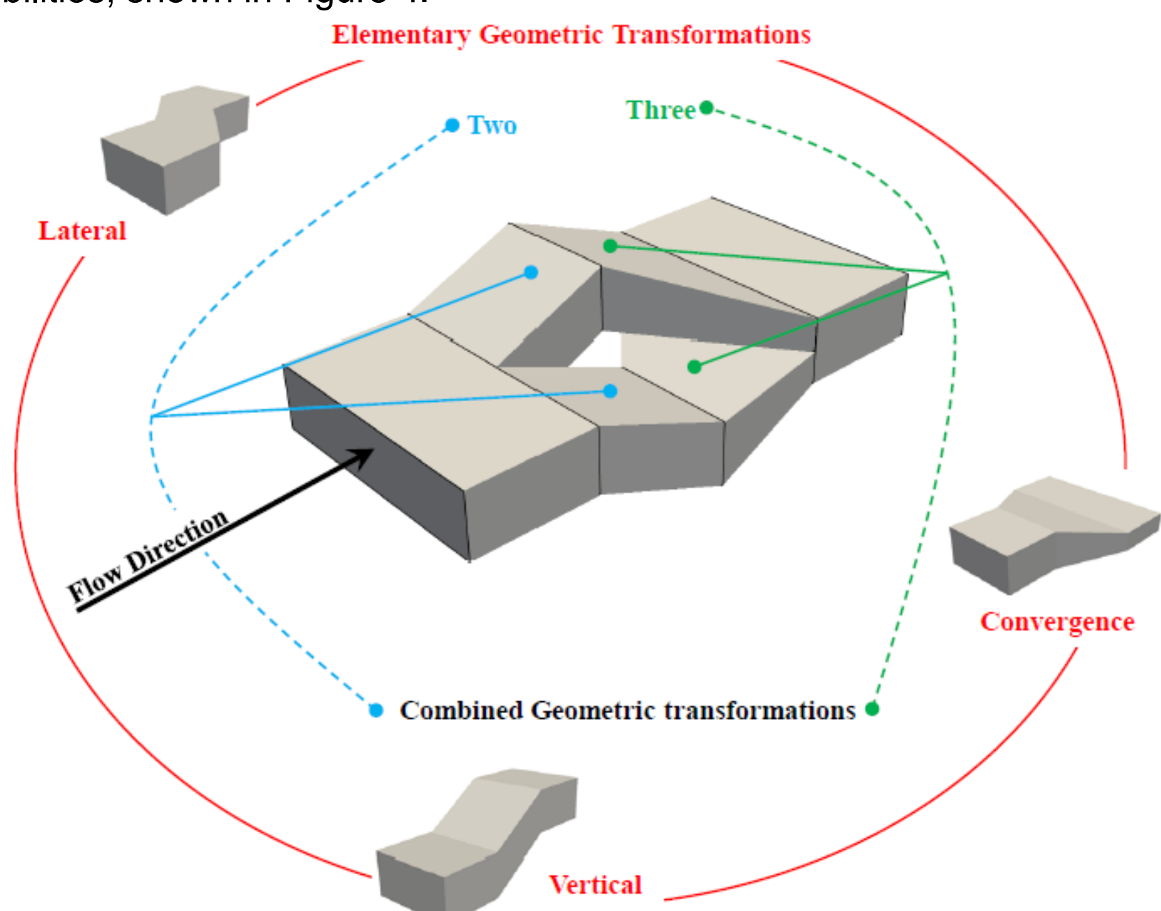
Figure 3. GTs present on Dooley's ISG die.
