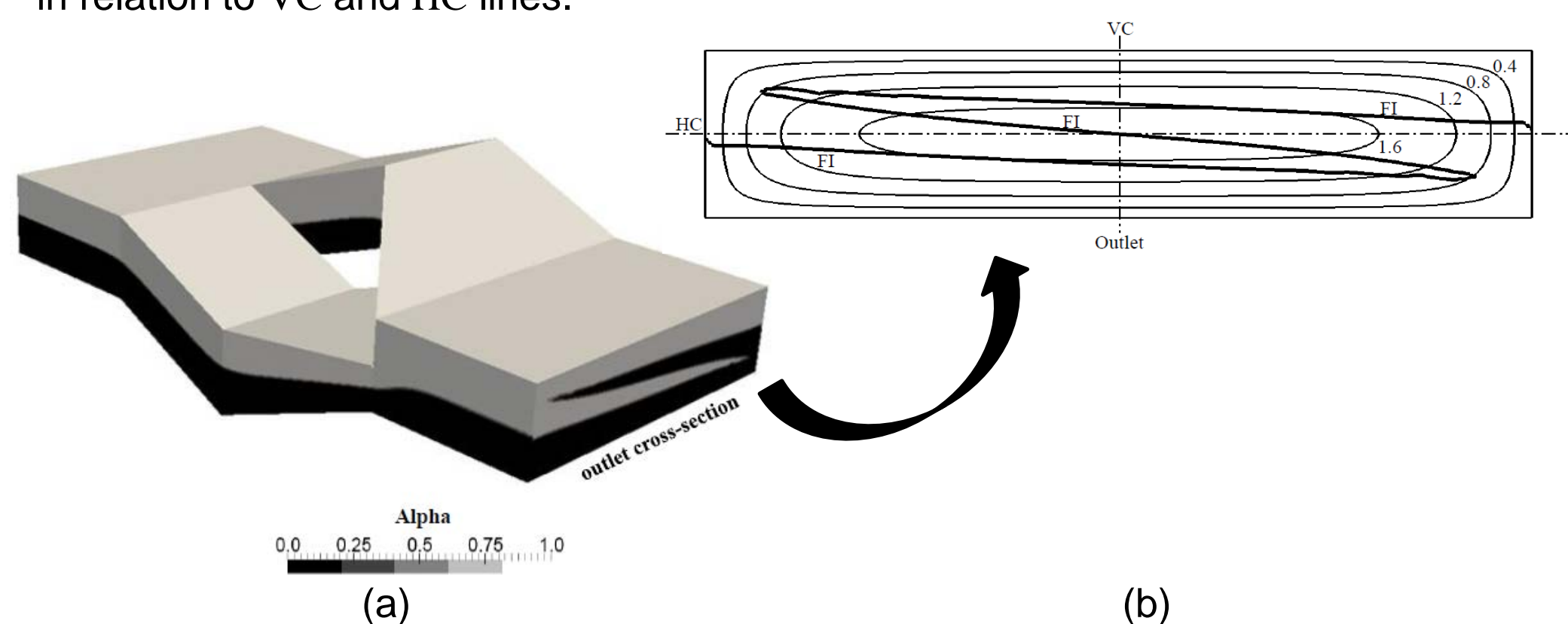
Figure 2. Dooley's ISG results. (a) Phase fraction. (b) Normalized velocity and interface contours.
