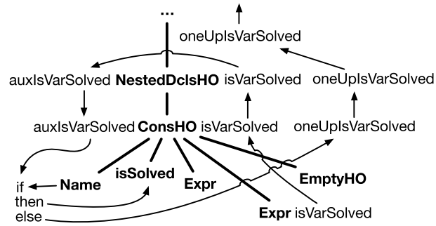
Fig. 4. Dependency between isVarSolved , isVarSolved_{aux} and oneUplIsVarSolved .
