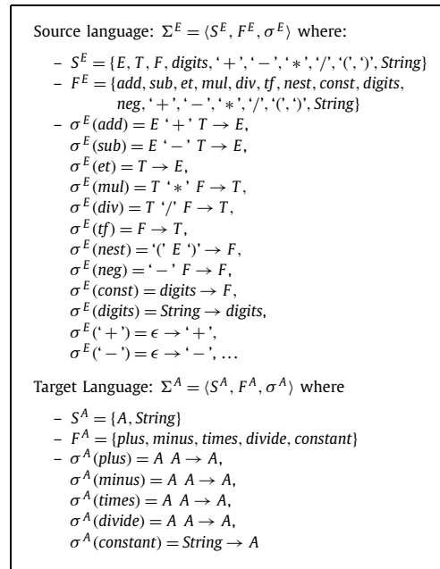
Fig. 5. Concrete and abstract syntax of arithmetic expressions.
