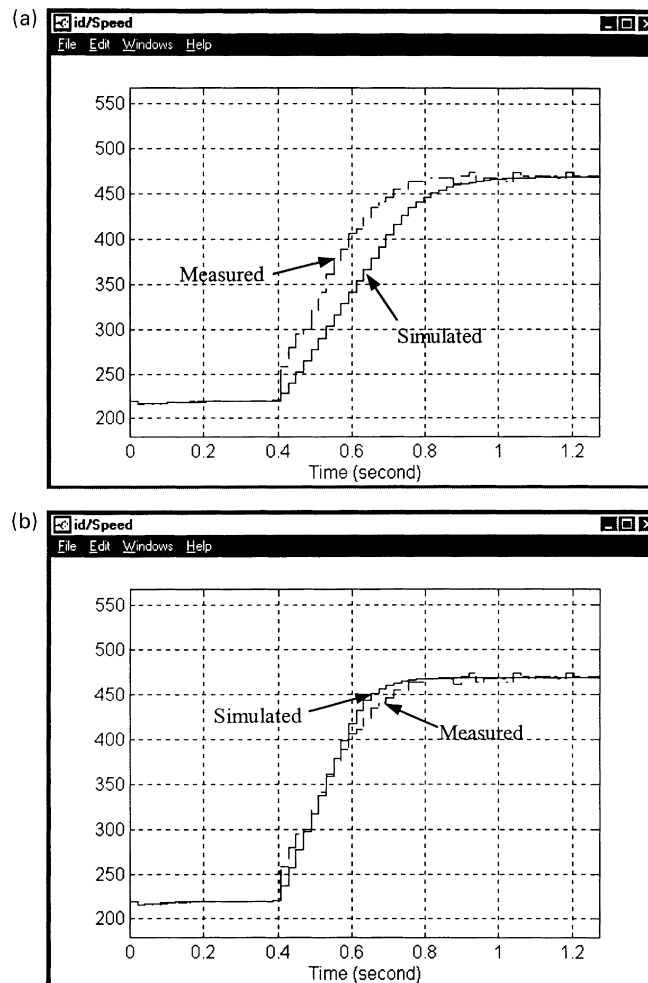
Fig. 7. Motor speed response: (a) measured and simulated data before the identification process; (b) measured and simulated data after the identification process.
