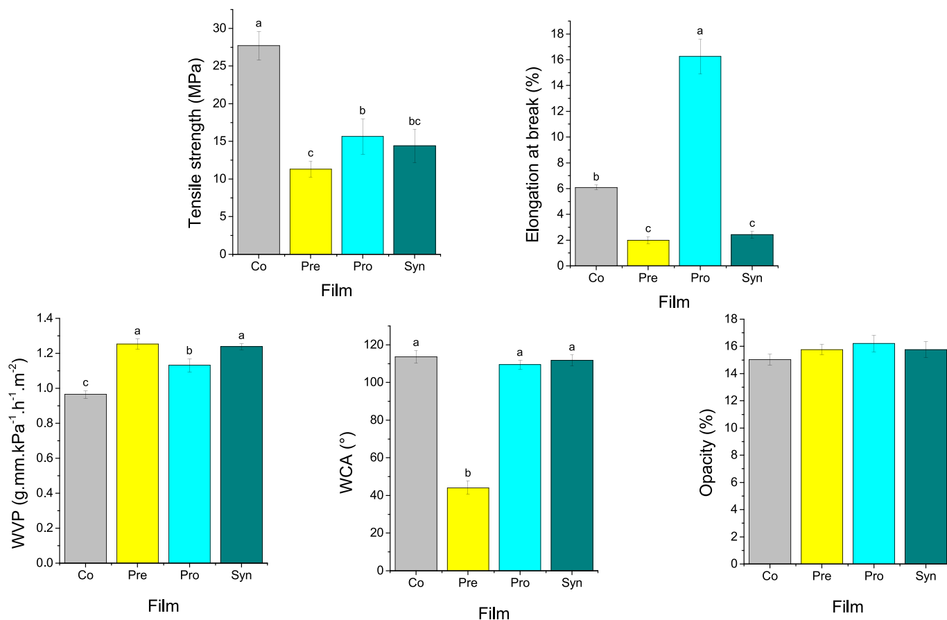
Fig. 1. Physical properties the films. WVP: water vapor permeability. WCA: water contact angle. Values in the same graph followed by at least one common letter (or not followed by any letters) are not significantly different ( p < 0.05 ).
