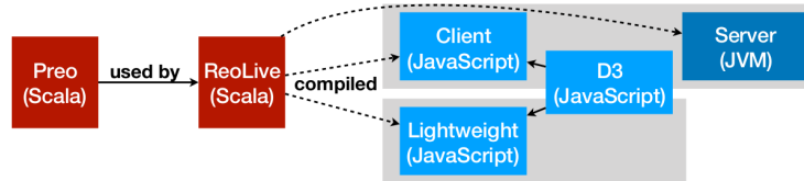
Figure 4.4: Architecture of the ReoLive implementation.
