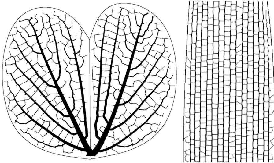
Figure 67: Left: Reticulate pattern (Orchid leaf); Right: Percurrent pattern (Grass leaf). Source: Runions et al. (2005)
