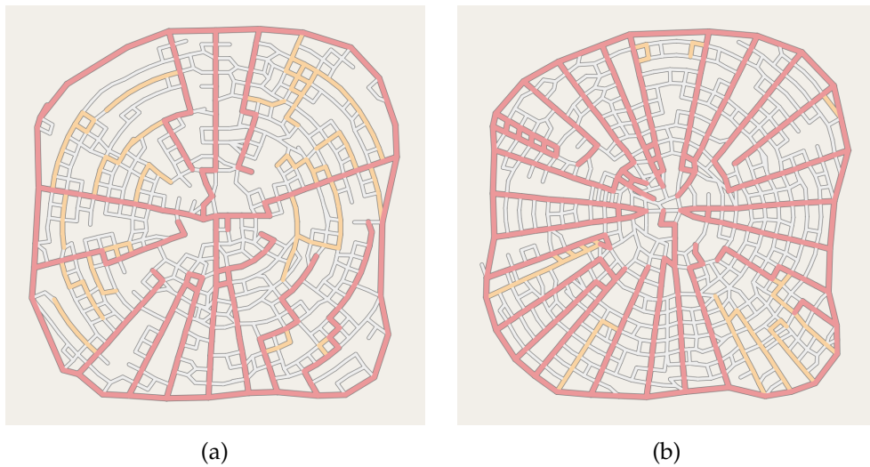
Figure 104: Radial road maps generated using different amounts of attraction points (per phase): a) 2500; b) 10000;
