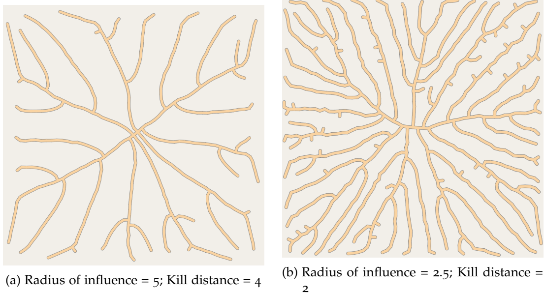
Figure 72: Capillarity of two maps with a kill distance and radius of influence ratio of 0.8.
