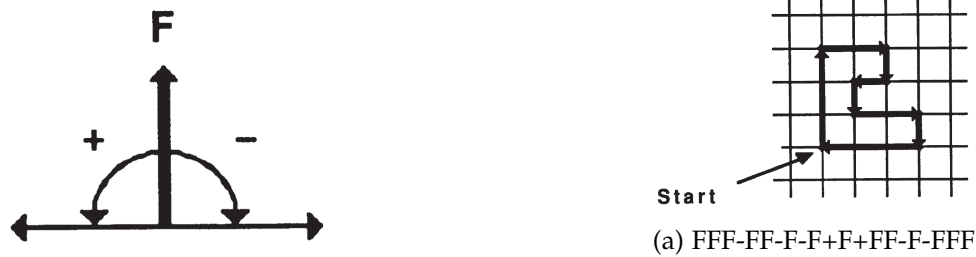
Figure 1: A turtle interpretation applied to a possible and simple L-System. Source: Prusinkiewicz and Lindenmayer (1990)
