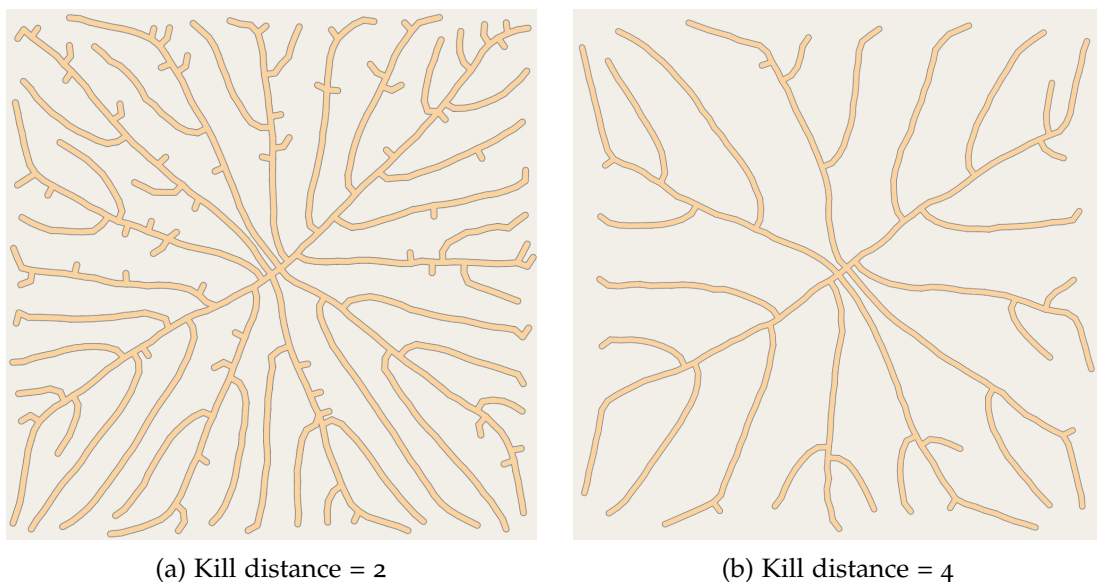
Figure 71: Capillarity influence result.
