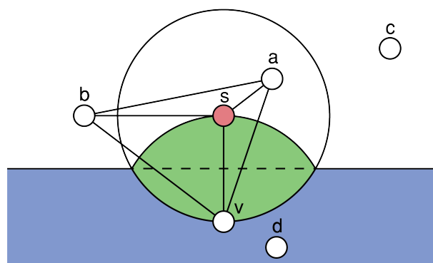
Figure 68: Relative neighbourhood example. Source: Runions et al. (2005)
