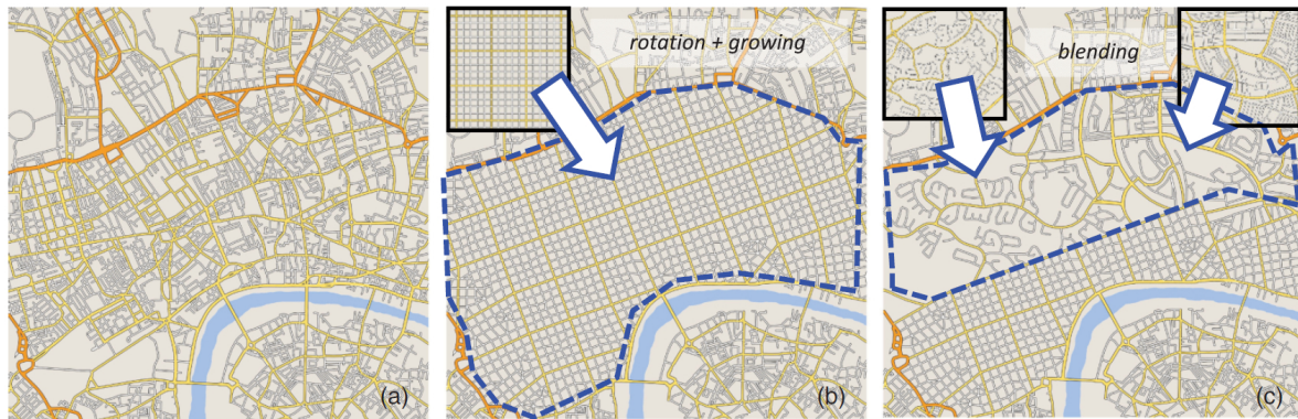
Figure 61: a) User-selected target area; b) Area replaced with a regular grid pattern; c) A more organic type of network was generated in the centre. Source: Nishida et al. (2016)
