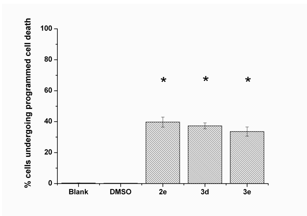
Figure 2. Analysis of programmed cell death of NCI-H460 cells treated with the compounds. Cells were treated for 24 h ( A ) or 48h ( B ) with medium, DMSO, or the
