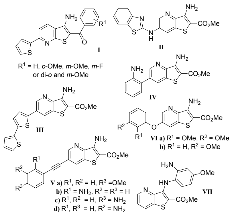
Structures of compounds I-VII
