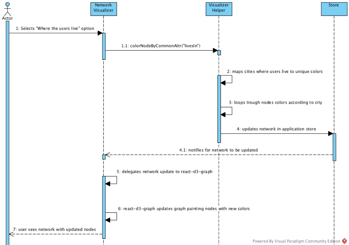
Figure 12: Socii sequence diagram community detection based on node properties.
