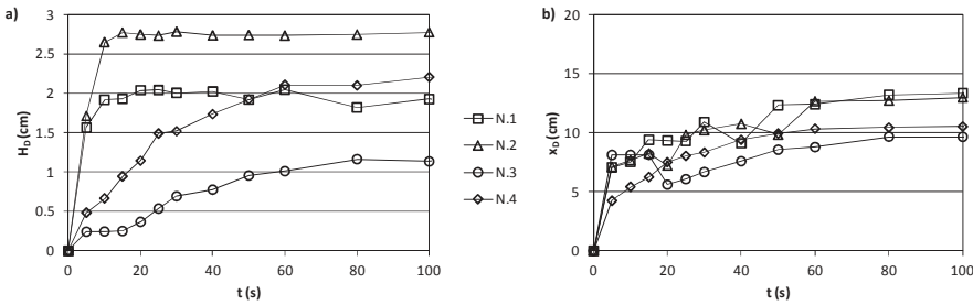
Fig. 7. Maximum dune height evolution with time (a) and corresponding longitudinal position (b). Only the first 100 s are presented since, afterwards, dune maximum height and location remain practically constant.
