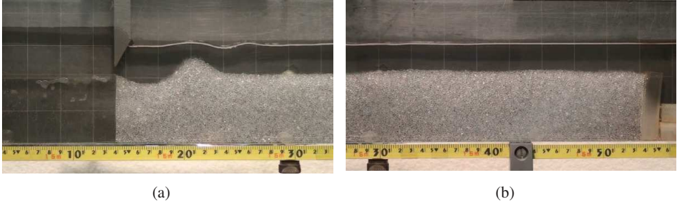
Fig. 2. Images of the initial (a) and final (b) part of the channel, obtained for the experimental condition N. 1 at time t = 5 s.
