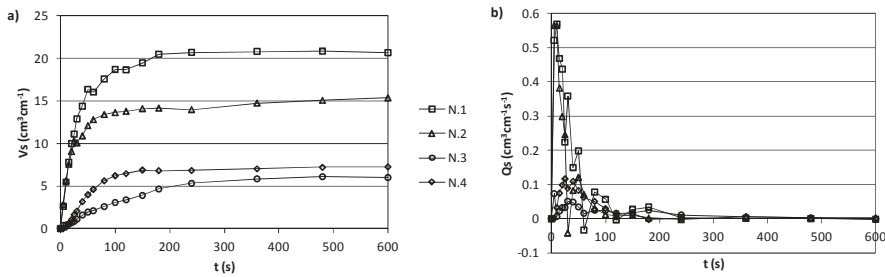
Fig. 9. Time evolution of the (a) scour volume per unit width and (b) solid transport rate per unit width.
