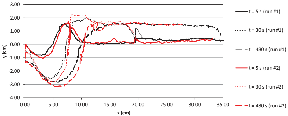
Fig. 8. Comparison of the sediment bed profiles in case of test condition N.1, for two different runs.
