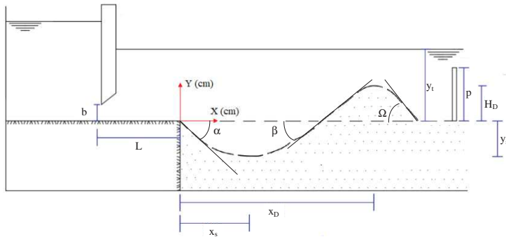
Fig. 1. Test section. y_s is the maximum scour depth and x_s is the corresponding x coordinate. H_D is the maximum dune height and x_D is the corresponding x coordinate. \alpha and \beta are the upstream and downstream slopes of the scour cavity, respectively. \Omega is the downstream slope of the dune.
