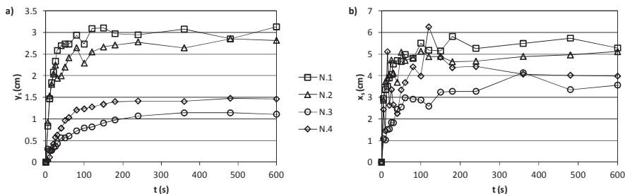
Fig. 6. Maximum scour depth evolution with time (a) and corresponding longitudinal position (b).
