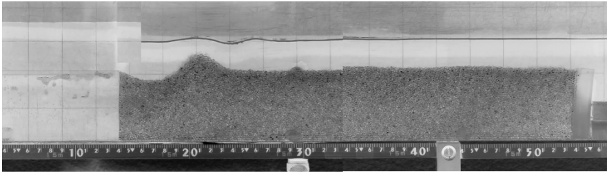
Fig. 3. Resulting full image, obtained for the experimental condition N. 1 at time t = 5 s.
