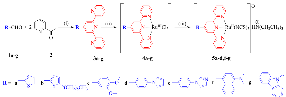
Scheme 1. Reagents and conditions for the synthesis of terpyridine ligands 3 , and complexes 4–5 : (i) EtOH, KOH, \text{NH}_3 \cdot \text{H}_2\text{O} , r.t; (ii) \text{RuCl}_3 , EtOH, \text{N}_2 ; (iii) DMF, KSCN, \text{H}_2\text{O} , TEA, reflux.
