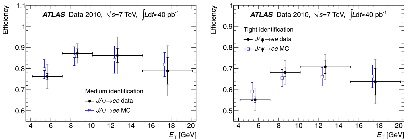
Fig. 17 Electron identification efficiencies measured from J/\psi \rightarrow ee events and predicted by MC for (left) medium and (right) tight identification as a function of E_T and integrated over |\eta| < 2.47 excluding the transition region 1.37 < |\eta| < 1.52 . The results for the data are shown with their statistical (inner error bars) and total (outer error bars) uncer-
