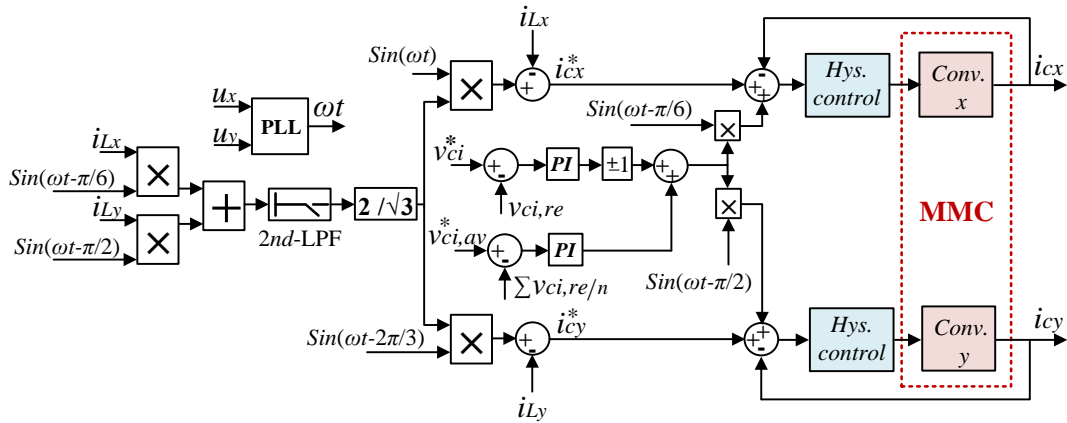
Fig. 4. Control strategy of the RPC based on an indirect MMC.
