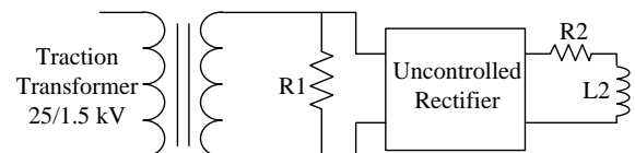
Fig. 5. Full locomotive model in PSIM .
