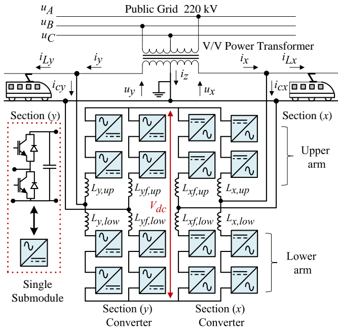
Fig. 1. RPC based on an indirect AC/DC/AC MMC connected to a V/V power transformer.
