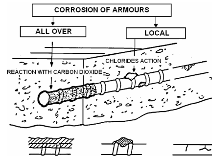
Fig. 1. Corrosion of steel armours
