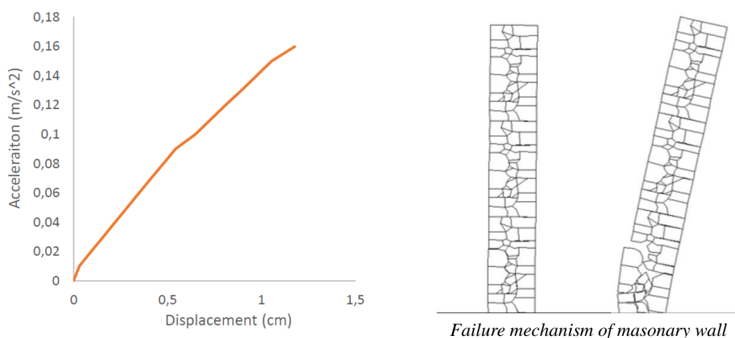
Fig. 11 Capacity curve of three-leaf masonry wall cross section and collapse mechanism subjected to out of plane loading.
