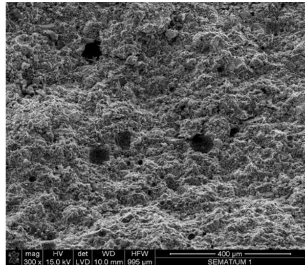
Fig. 4. The microstructure of concrete with 1% resin
