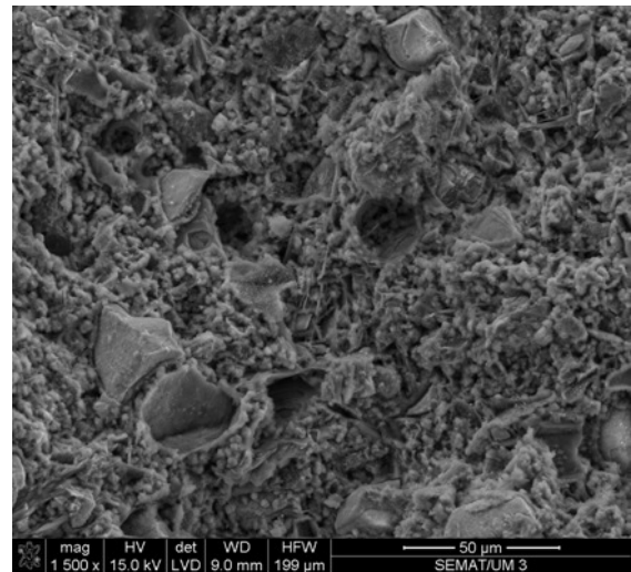
Fig. 5. The microstructure of concrete with an epoxy resin proportion of 5%
