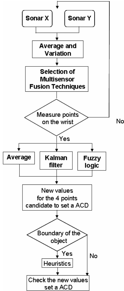
Fig. 5. Flowchart of the sensor fusion process
