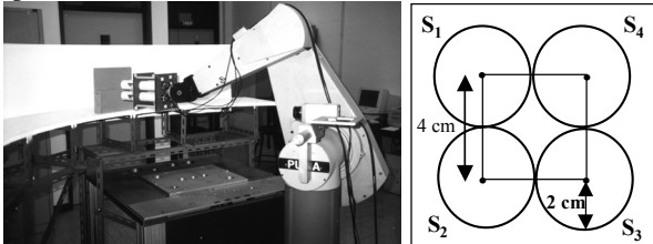
Fig. 2. Work cell
