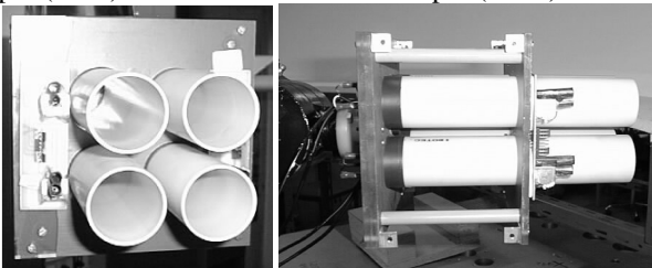
Fig. 4. Detail of the sonars on the wrist
