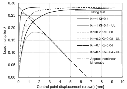
Figure 6. Arch capacity curves varying the interface stiffness.
