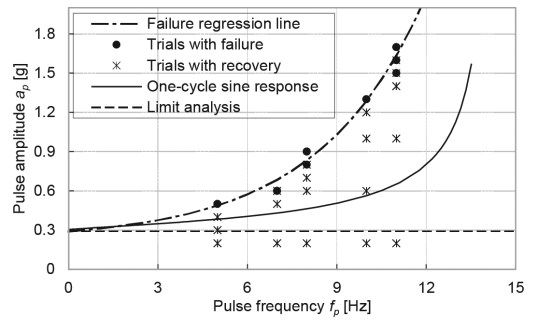
Figure 5. Results of the shaking table tests.
