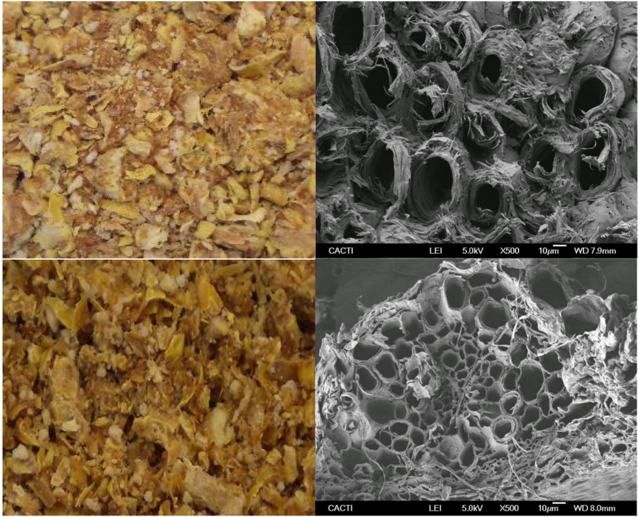
Fig. 4 Visual aspect and SEM photographs showing the morphology of lignocellulosic surface of a raw corncob, b destarched corncob, c destarched corncob followed by NaOH treatment, d destarched corncob followed by NH 4 OH treatment, e destarched corncob treated by autoclave, and f destarched corncob treated by autoclave and microwave
