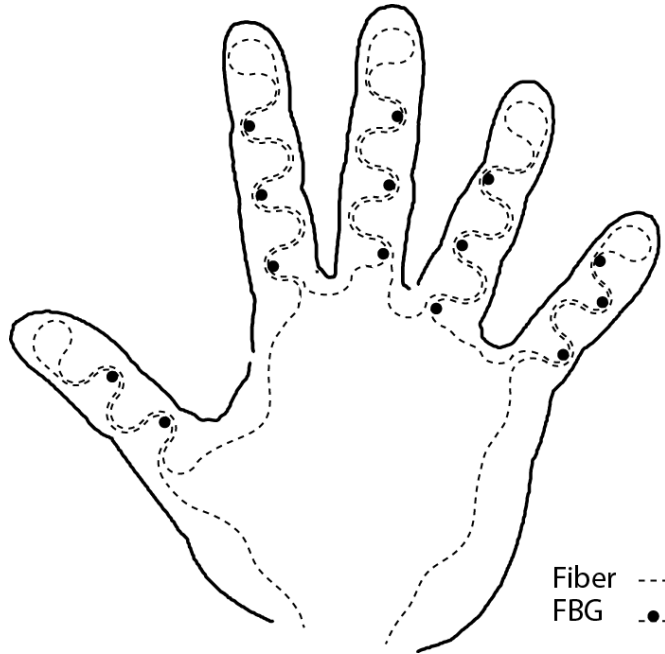
Figure 6. FBG sensor positioning proposal.
