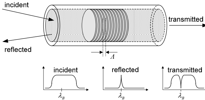
Figure 1. Illustration of working principle of FBGs.
