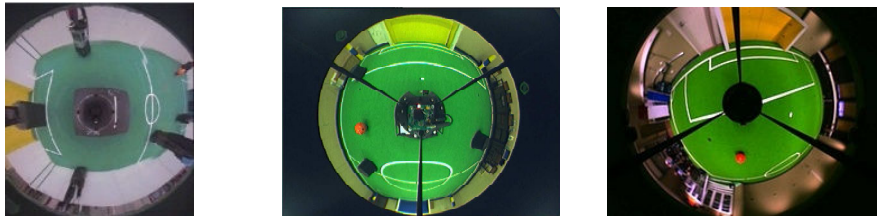
Fig. 1- Three examples of images captured by a catadioptric vision system from different MSL teams. Left – MRT team [1], Centre – Cambada [2], Right – Brainstormers Tribots [3]
