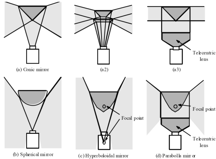
Fig. 3 – Different omnidirectional mirrors [10]
