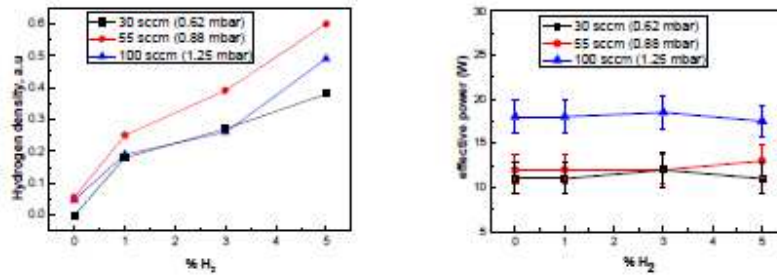
Fig.1 H atoms relative density (left) and effective RF power coupled to the plasma (right), as a function of the concentration of molecular hydrogen, at V_{rf}=220V and for various pressures.
