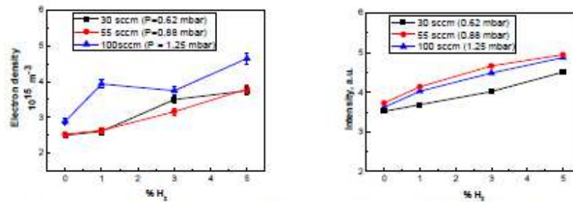
Fig. 2 Electron density (left) and intensity of the FNS band of N_2^+ , (right), as a function of the concentration of molecular hydrogen, at V_{rf}=220V and for various pressures.
