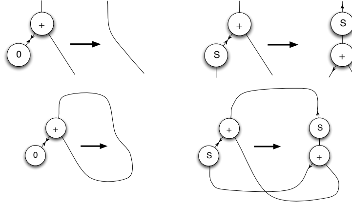
Fig. 2. Interaction rules for natural number arithmetics (top), and the same rules represented as the nets \langle +(x, x), 0 \rangle and \langle +(S(y), x), S(+ (y, x)) \rangle (bottom)
