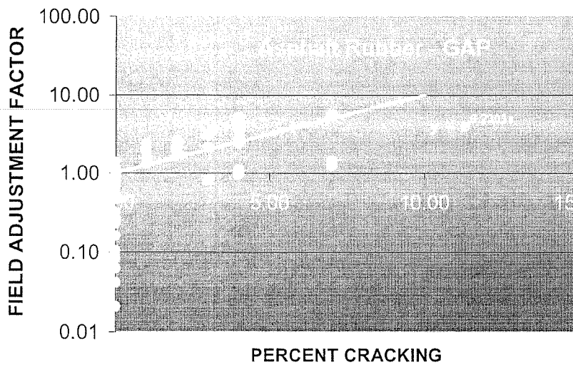
Figure 6 – Relationship Between FAF and Percent Cracking for Asphalt Rubber Gap-Graded Sections.
