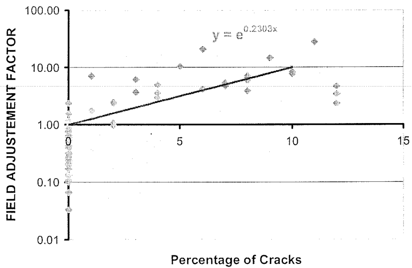
Figure 8 – Comparison Between Modeled and Predicted Number of ESALs to the Reported Crack Level for all Pavement Sections in the Database (Conventional and Asphalt Rubber).
